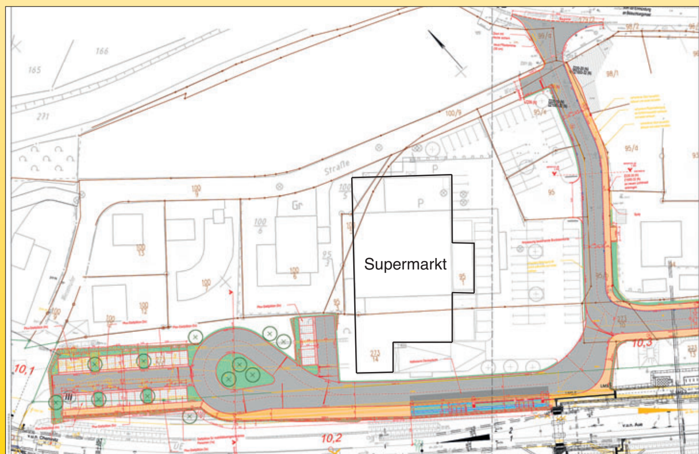
Bauplan Buswendeschleife
